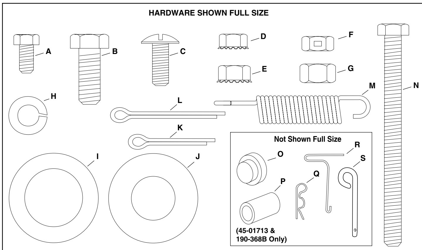
FIGURE 1 - HARDWARE PACK
